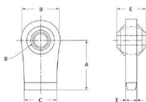
LIFT ARM END (STRAIGHT)
